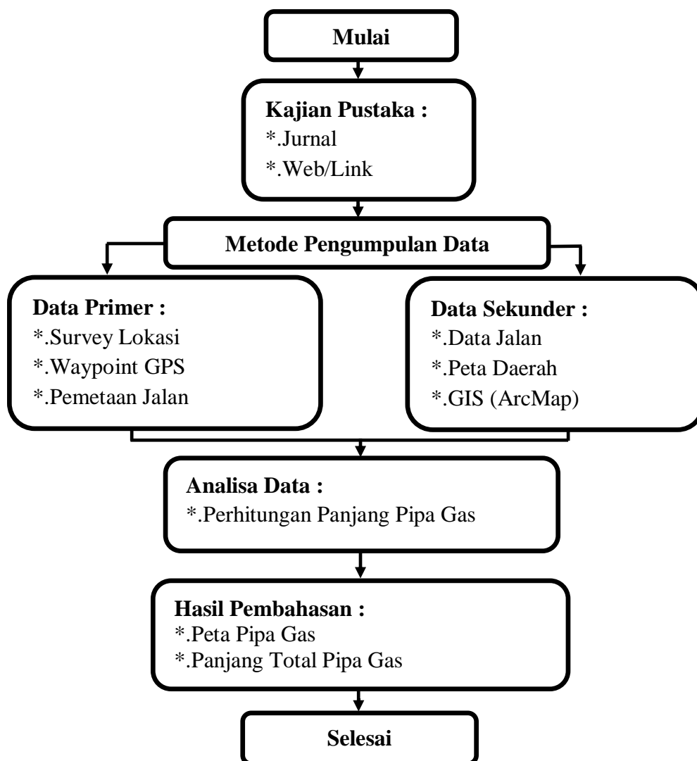
Gambar 3.1 Alur Penelitian
